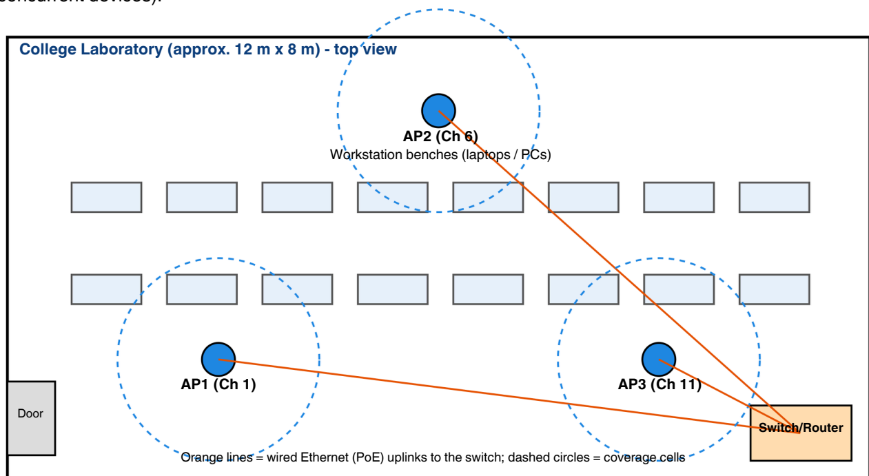
Figure 3: Proposed WLAN layout with three access points on non-overlapping channels.
