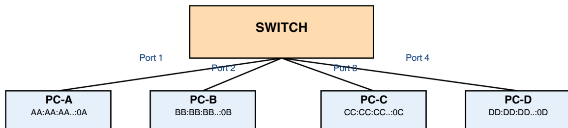
Figure 2: Example LAN with four hosts connected to one switch.
